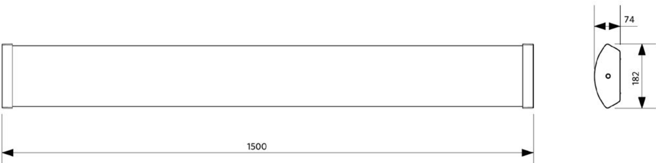
LEDLinear-E CL15
