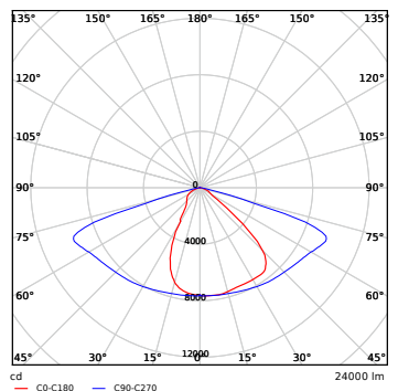
LEDRoadlight-200W
