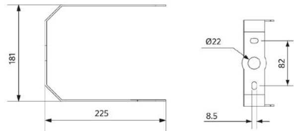
LEDHighbay-P4 Bracket-D420
