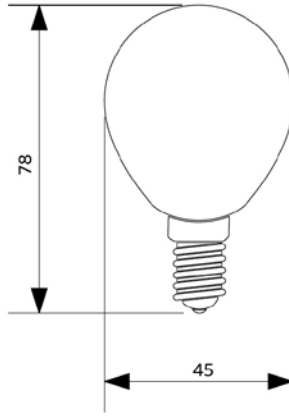
LED-E-P45-FILA
