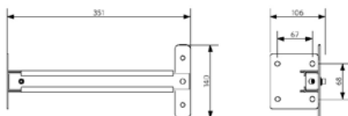
LED Flood-E-Re250-280-Bracket
