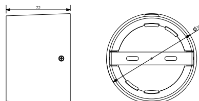
560098000600 - LEDsmart-Sensor Surface-Module-WH
