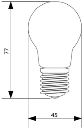
LED-E-G45-FILA
