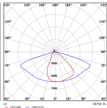
LEDRoadlight-150W
