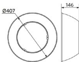
LEDHighbay-E2 Bracket-L249
