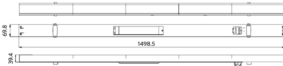
LEDTrunking Trunk 8
