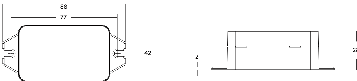
821017001300 - LEDSmart-BLE-DALI-Converter
