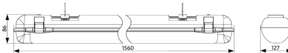
LEDWaterproof-CLA-E L1550
