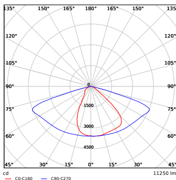
LEDRoadlight-90W
