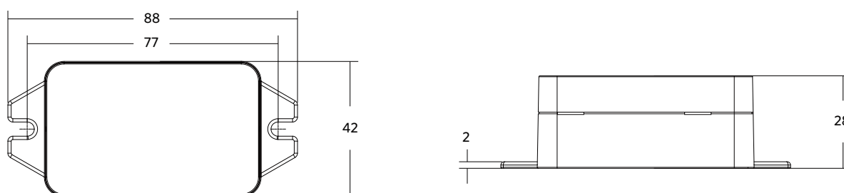
821017001400 - LEDSmart-BLE-10V-Converter
