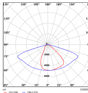
LEDRoadlight-120W
