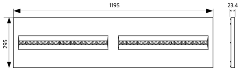
LEDPanelRc-Sy Re295
