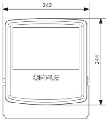
LED Flood-E-Re250-280-Bracket
