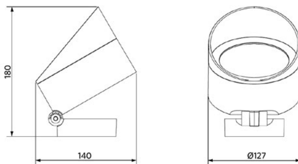
LEDSpotProjector-E Rd127
